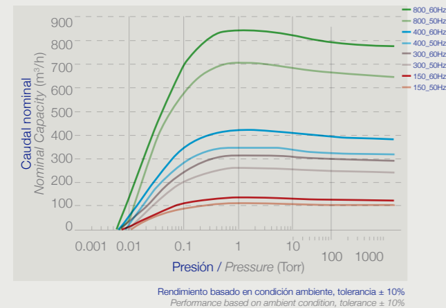
Curvas de caudal / Flow curves RVS-150/300/400/800
